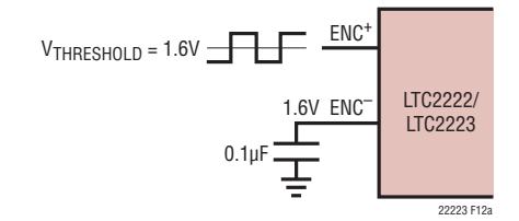
Figure 12a. Single-Ended ENC Drive, Not Recommended for Low Jitter
